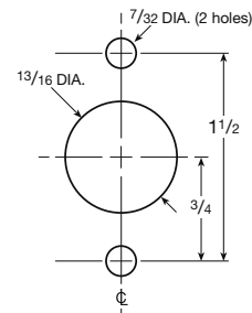
Mounting Hole Locations for 1000/1001
