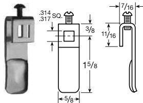
Cam No. S14452 Wrought Steel Zinc Plated
