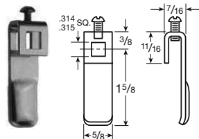
Cam No. S14441 Wrought Steel Zinc Plated
